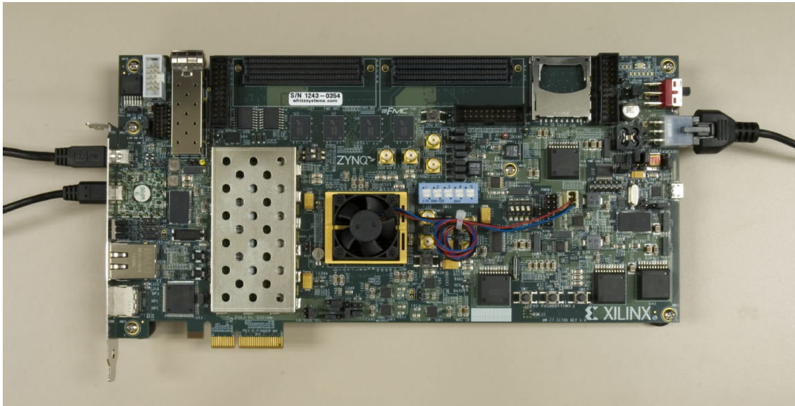
Figure 2-3: ZC706 Board with the UART and Power Cables Attached
