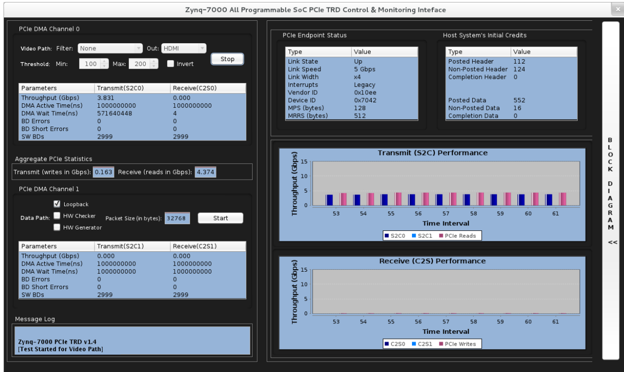
Figure 3-14: Performance Mode GUI
